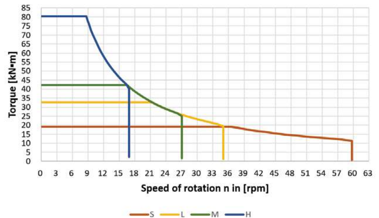
Rotary head
